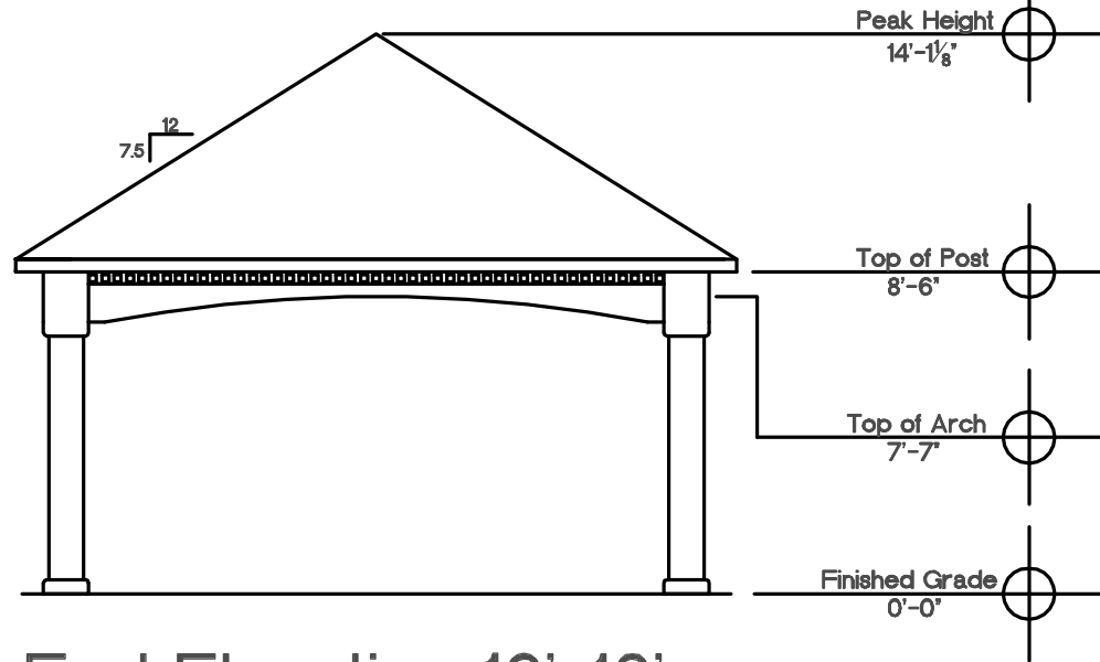
End Elevation 16'x16'
