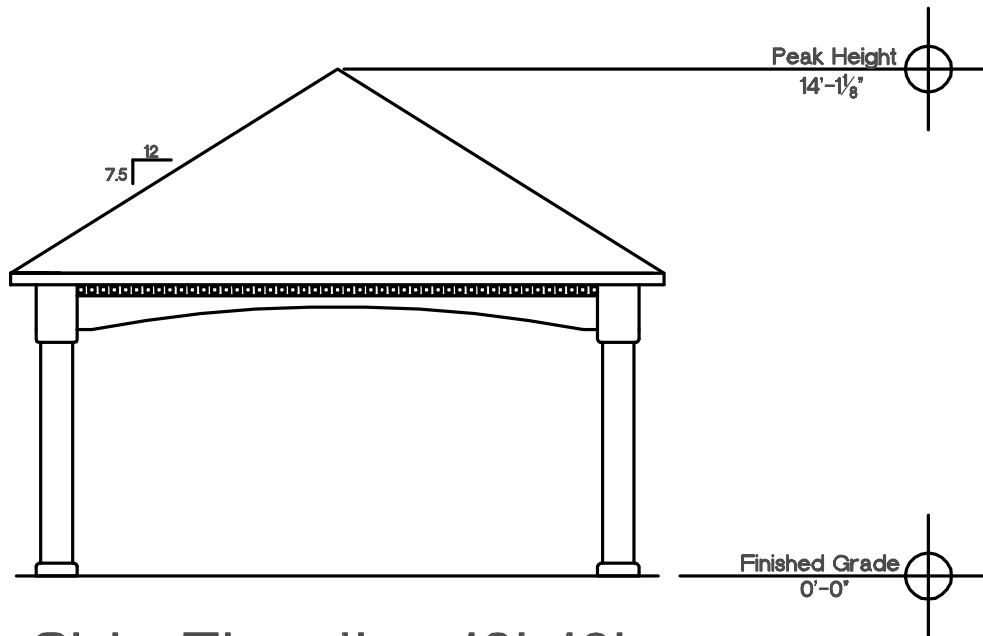
Side Elevation 16'x16'
