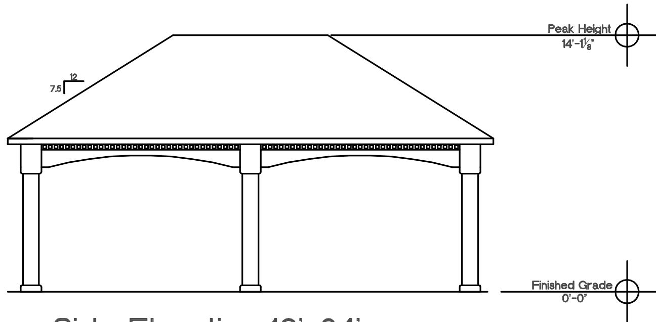
Side Elevation 16'x24'
