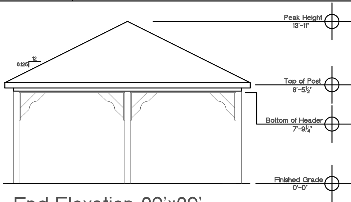
End Elevation 20'x20'
