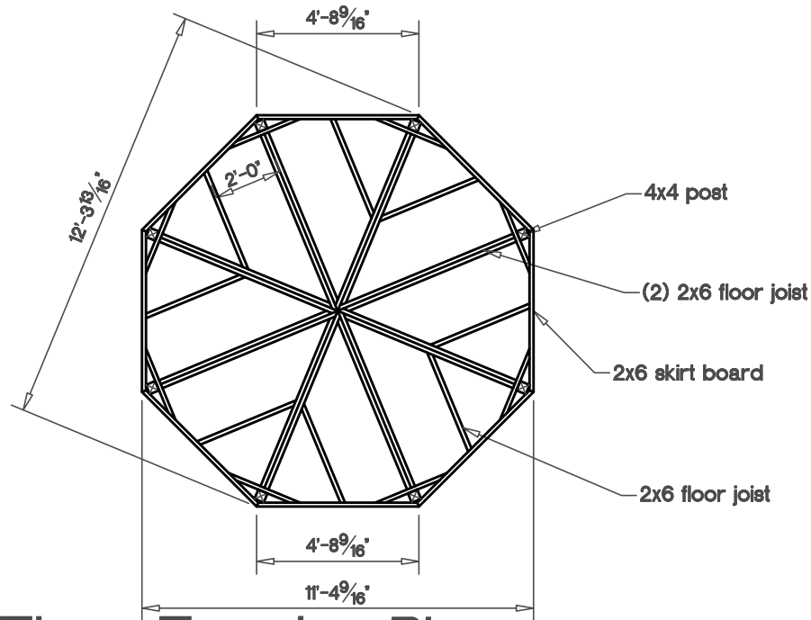
Floor Framing Plan Fully Assembled Unit
