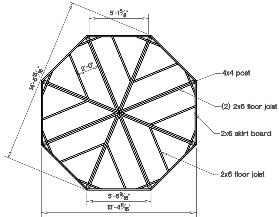
Floor Framing Plan Fully Assembled Unit
