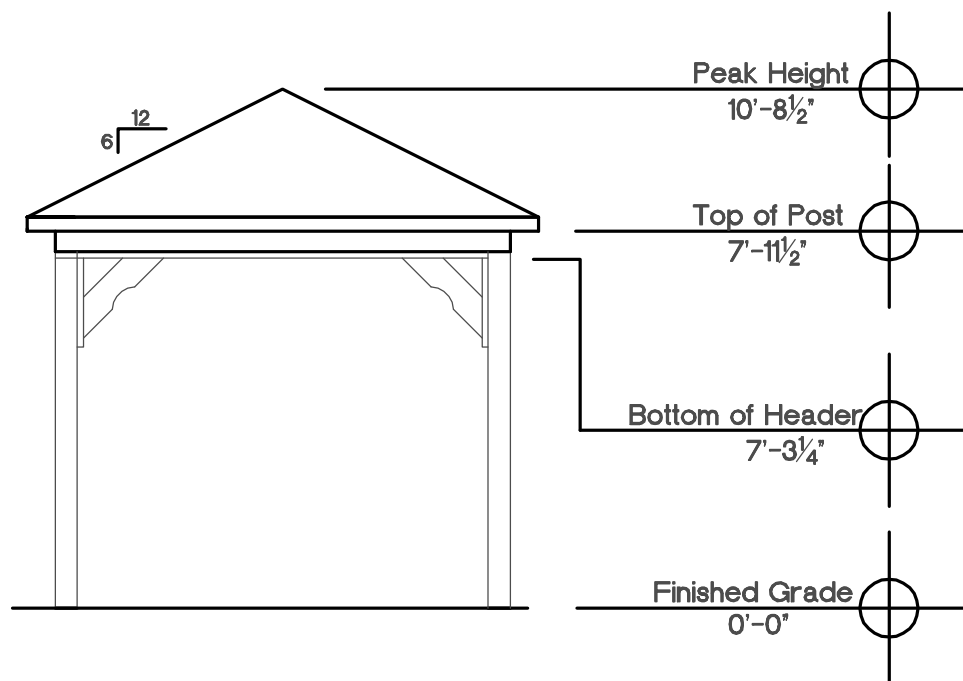
End Elevation 10'x14' Scale \frac{1}{4}'' = 1'-0''
