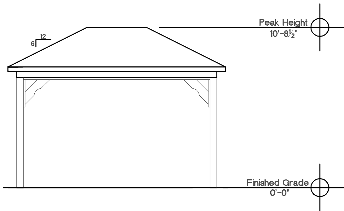
Side Elevation 10'x14' Scale \frac{1}{4}'' = 1'-0''
