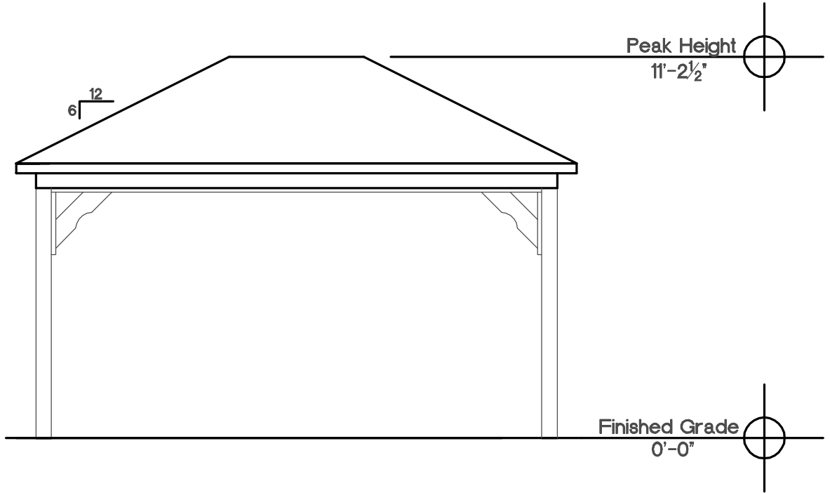
Side Elevation 12'x16' Scale \frac{1}{4}'' = 1'-0''
