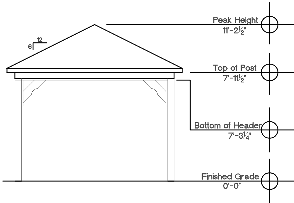
End Elevation 12'x16' Scale \frac{1}{4}'' = 1'-0''
