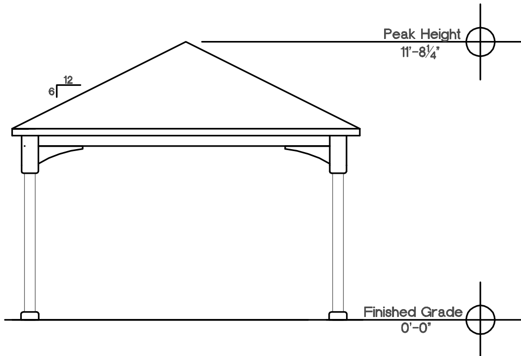
Side Elevation 14'x14'
