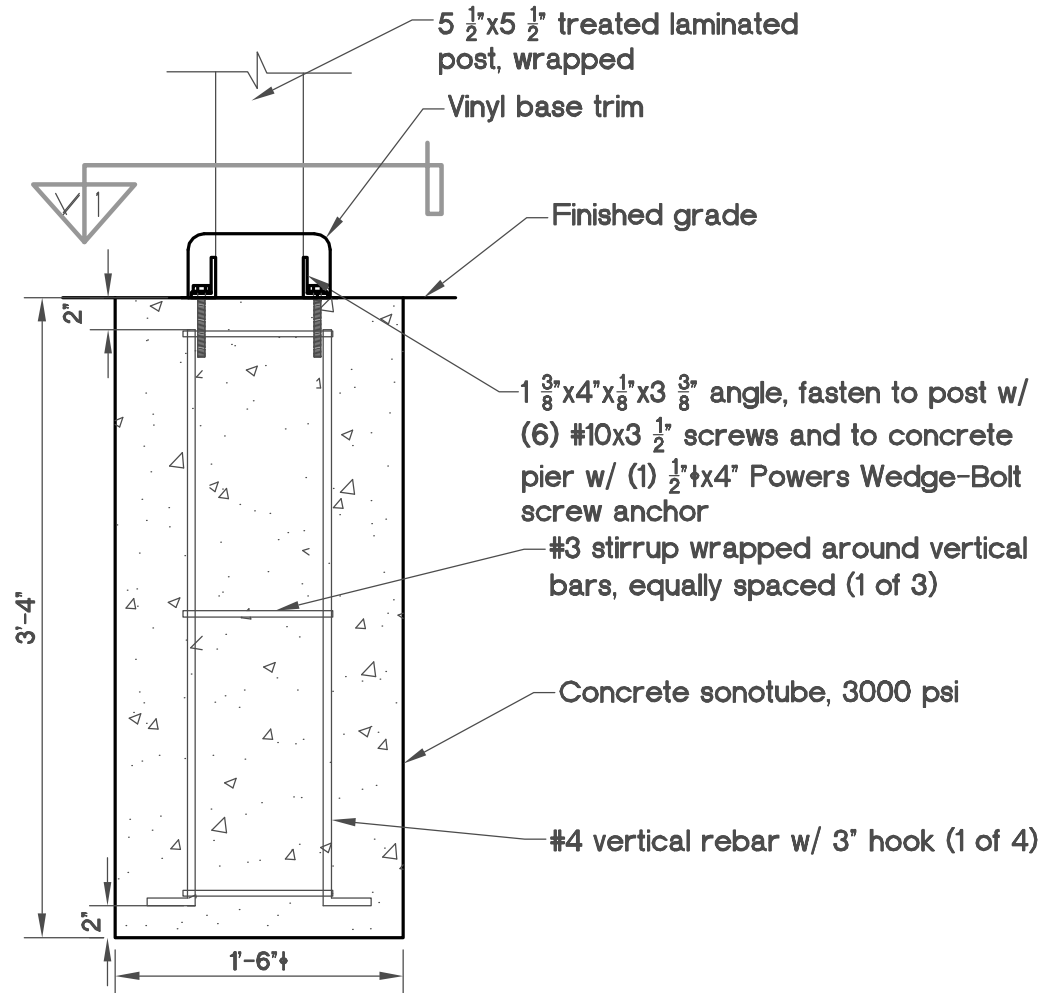
Pier Concept
