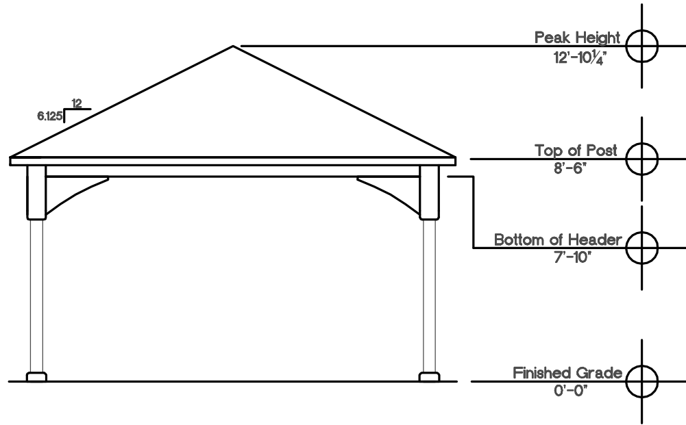
End Elevation 16'x16' NTS
