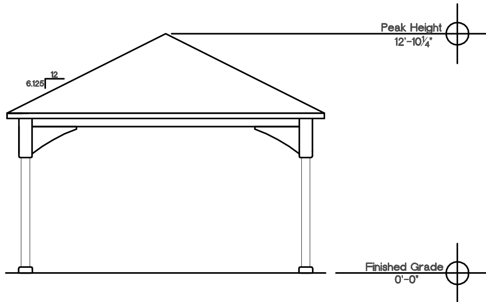
Side Elevation 16'x16' NTS
