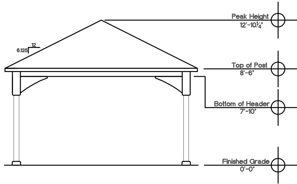
End Elevation 16'x18' NTS
