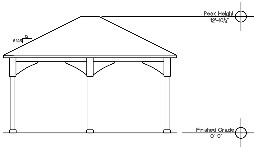
Side Elevation 16'x18' NTS
