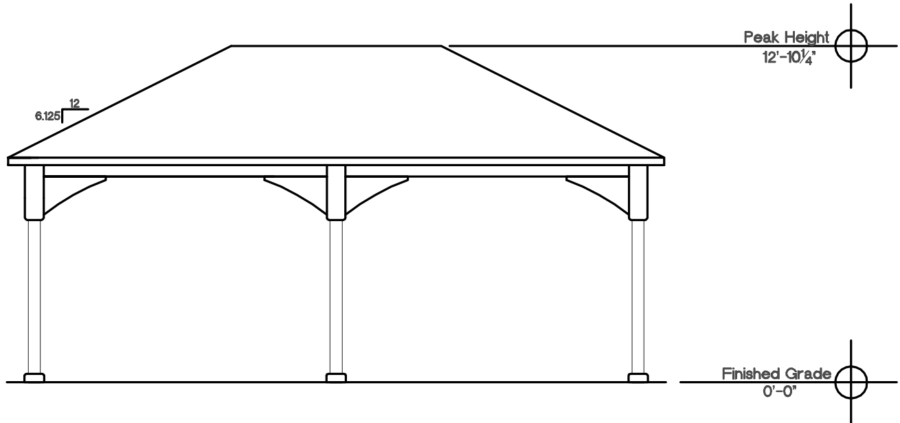
Side Elevation 16'x24' NTS
