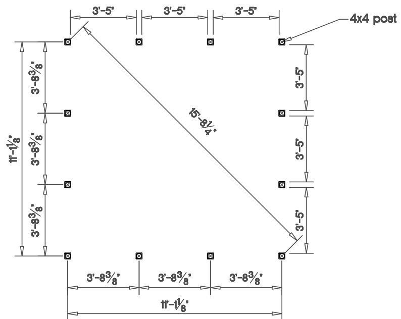
Post Layout Plan
