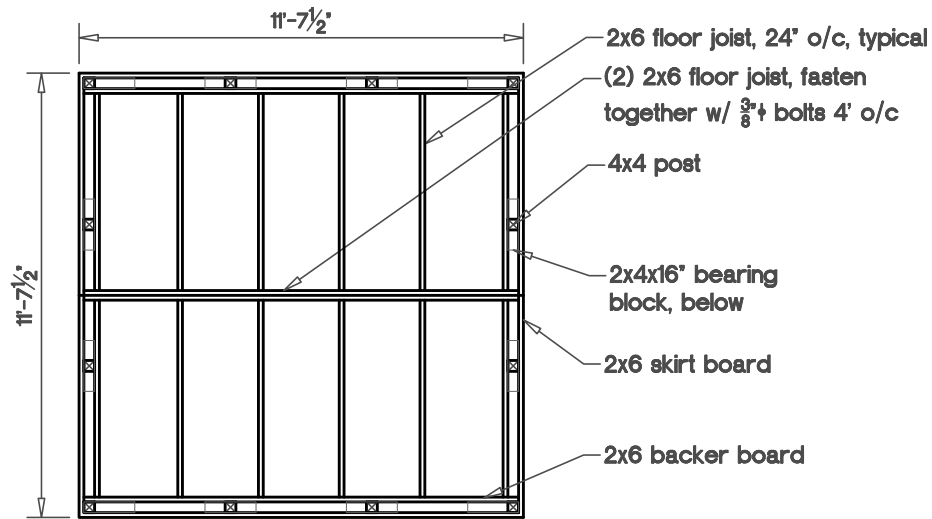
Floor Framing Plan Kit Unit
