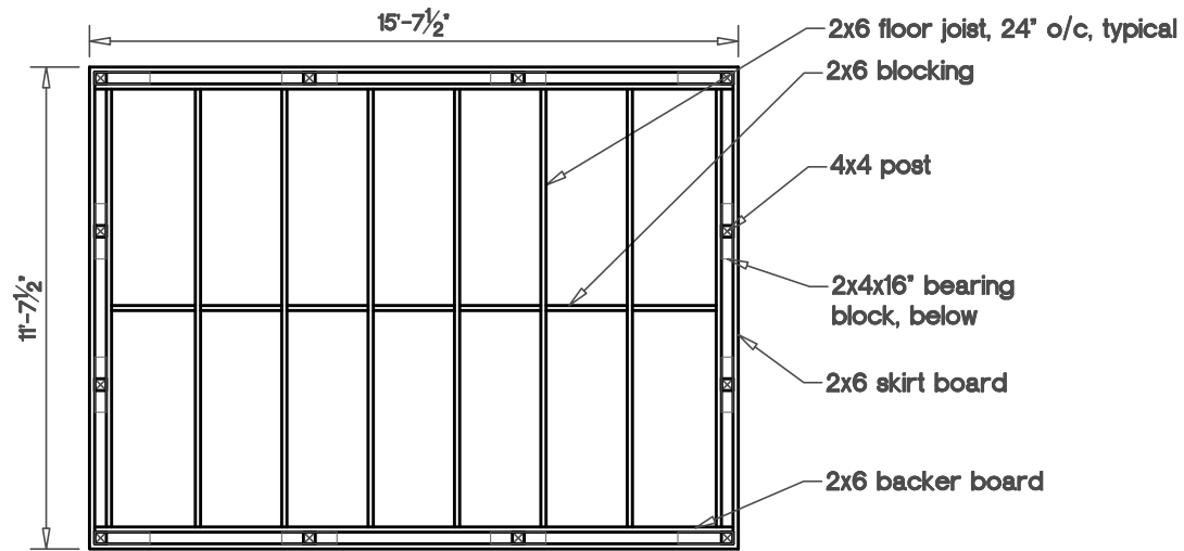
Floor Framing Plan Fully Assembled Unit
