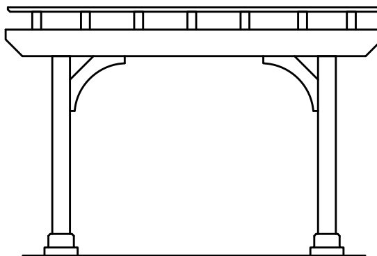
Side Elevation
