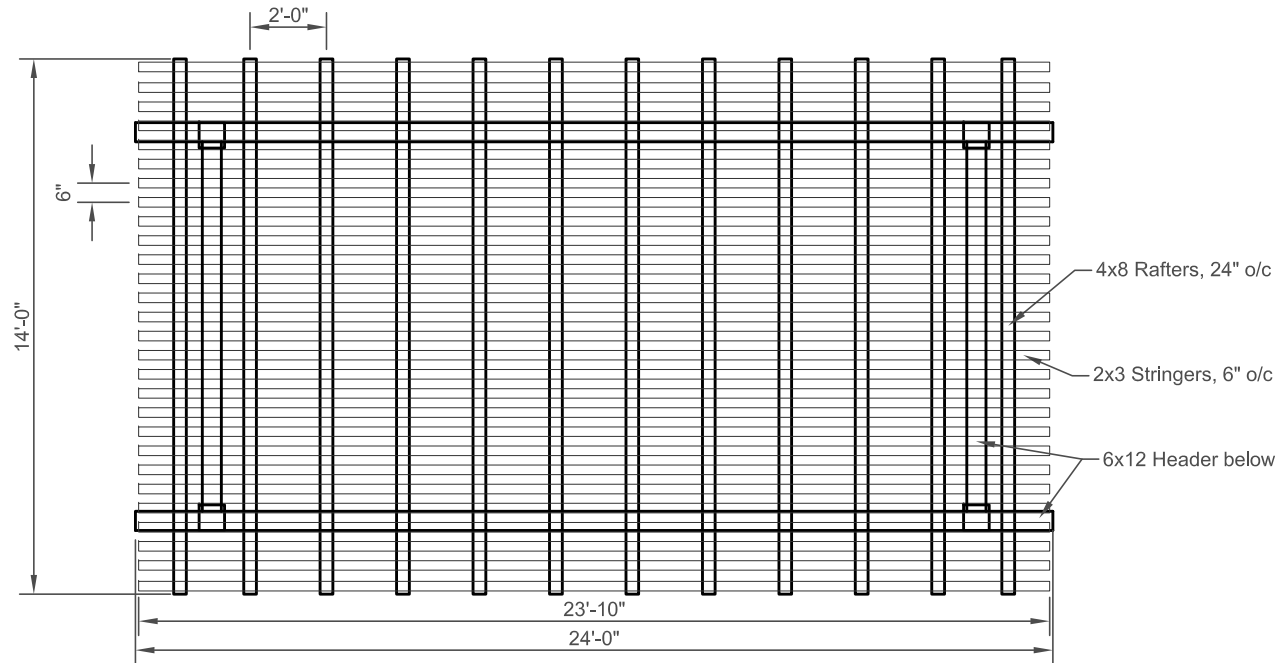
Roof Framing Plan
