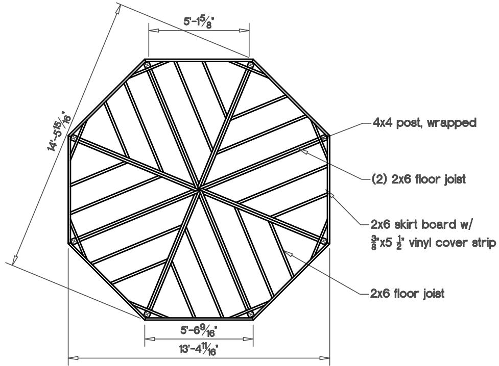
Floor Framing Plan Fully Assembled Unit
