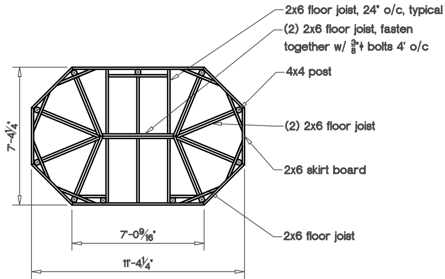
Floor Framing Plan Fully Assembled Unit
