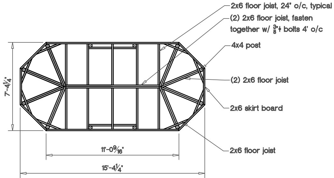
Floor Framing Plan Fully Assembled Unit
