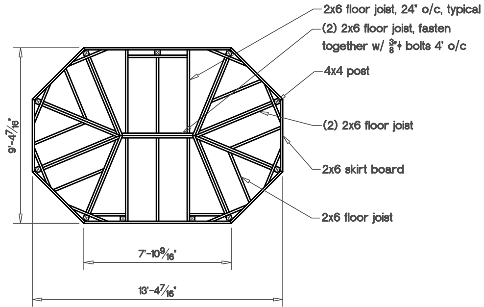
Floor Framing Plan Fully Assembled Unit
