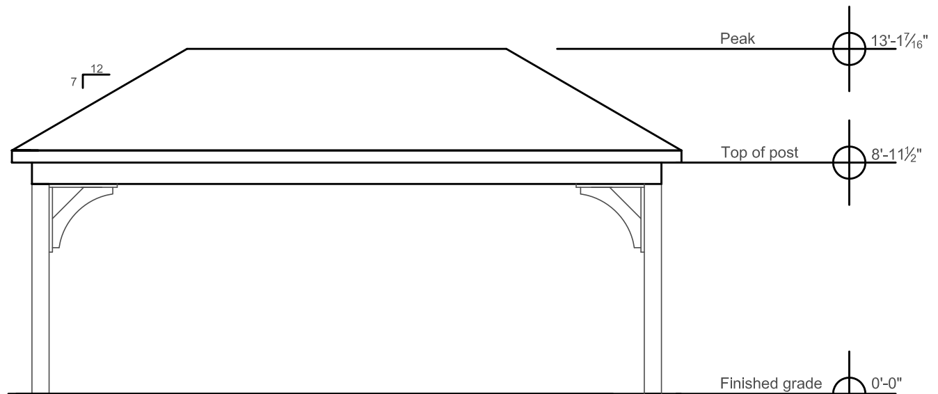
Side Elevation
