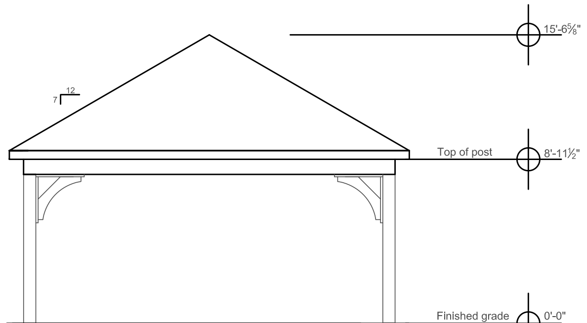
Side Elevation
