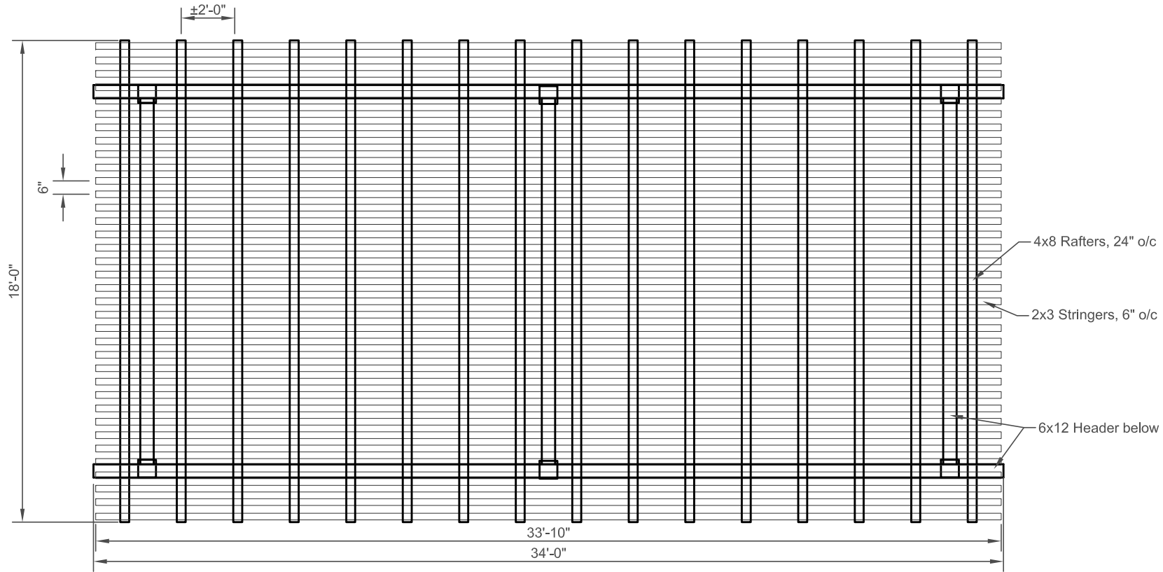
Roof Framing Plan
