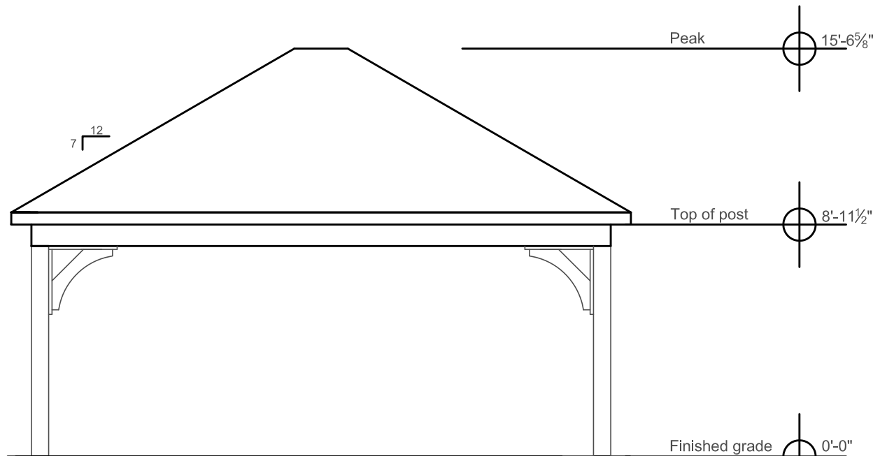
Side Elevation
