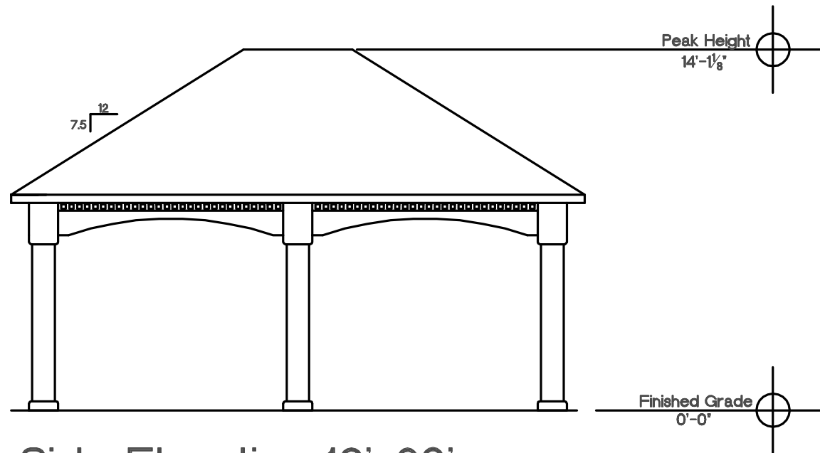
Side Elevation 16'x20'
