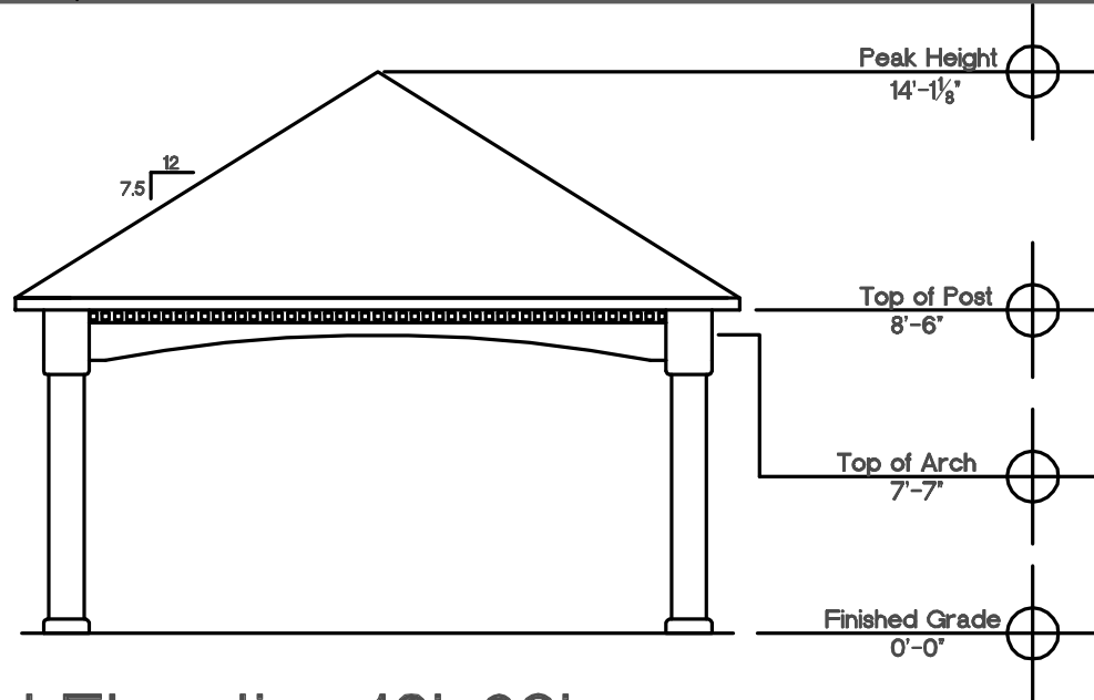
End Elevation 16'x20'
