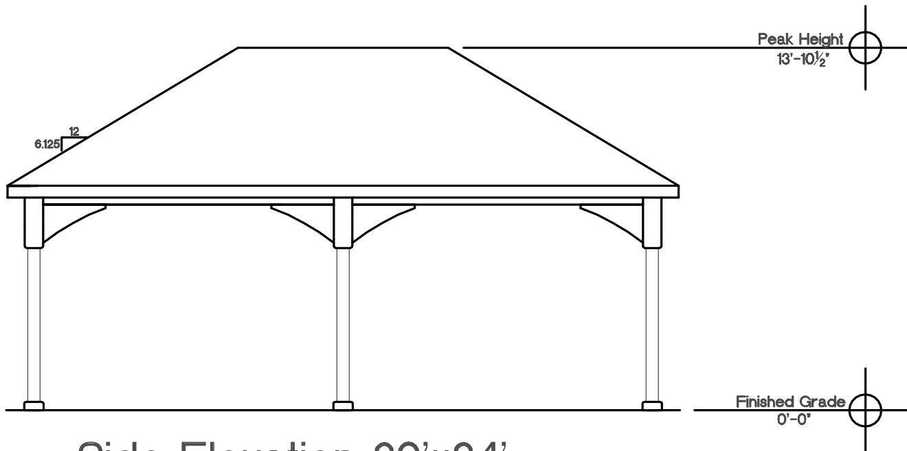
Side Elevation 20'x24' NTS
