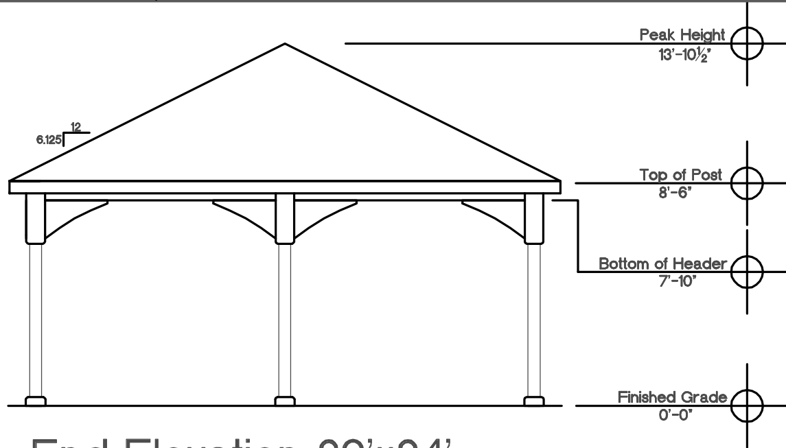
End Elevation 20'x24' NTS
