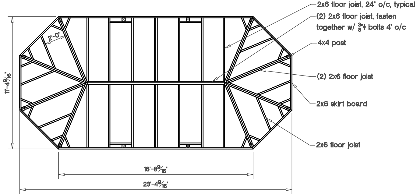
Floor Framing Plan Kit Unit
