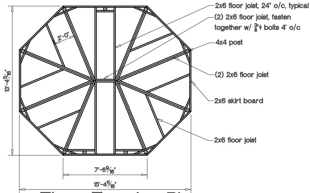
Floor Framing Plan Fully Assembled Unit
