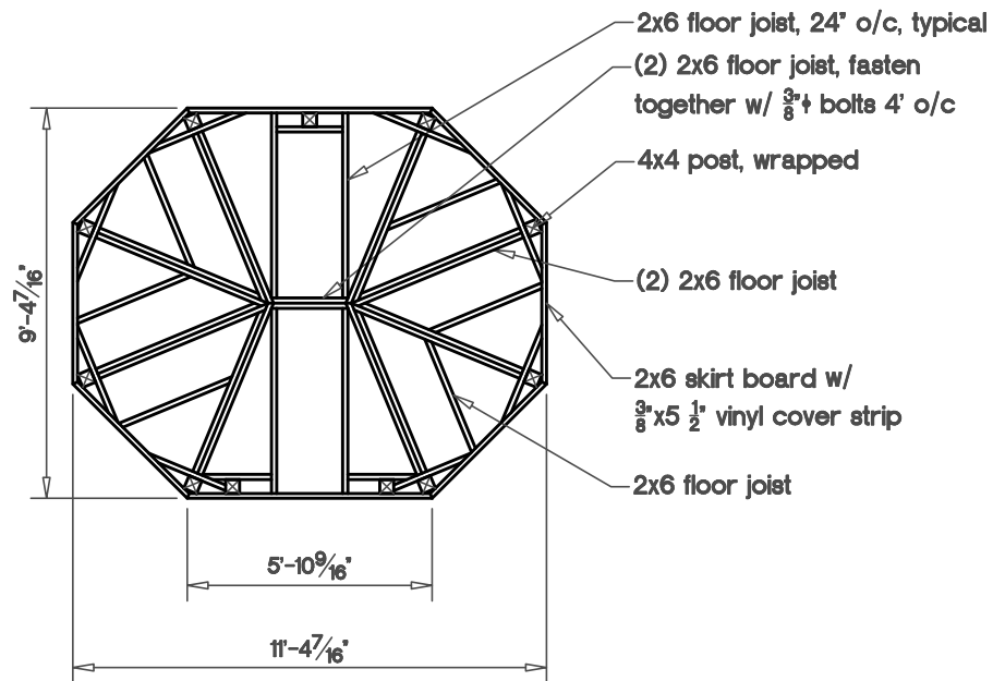
Floor Framing Plan Fully Assembled Unit
