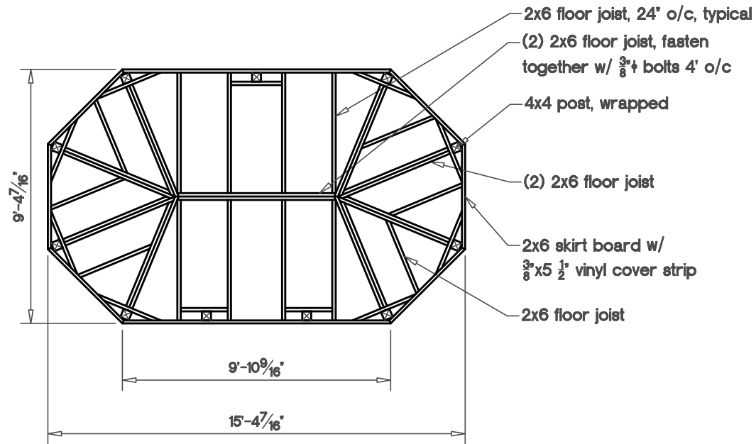
Floor Framing Plan Fully Assembled Unit
