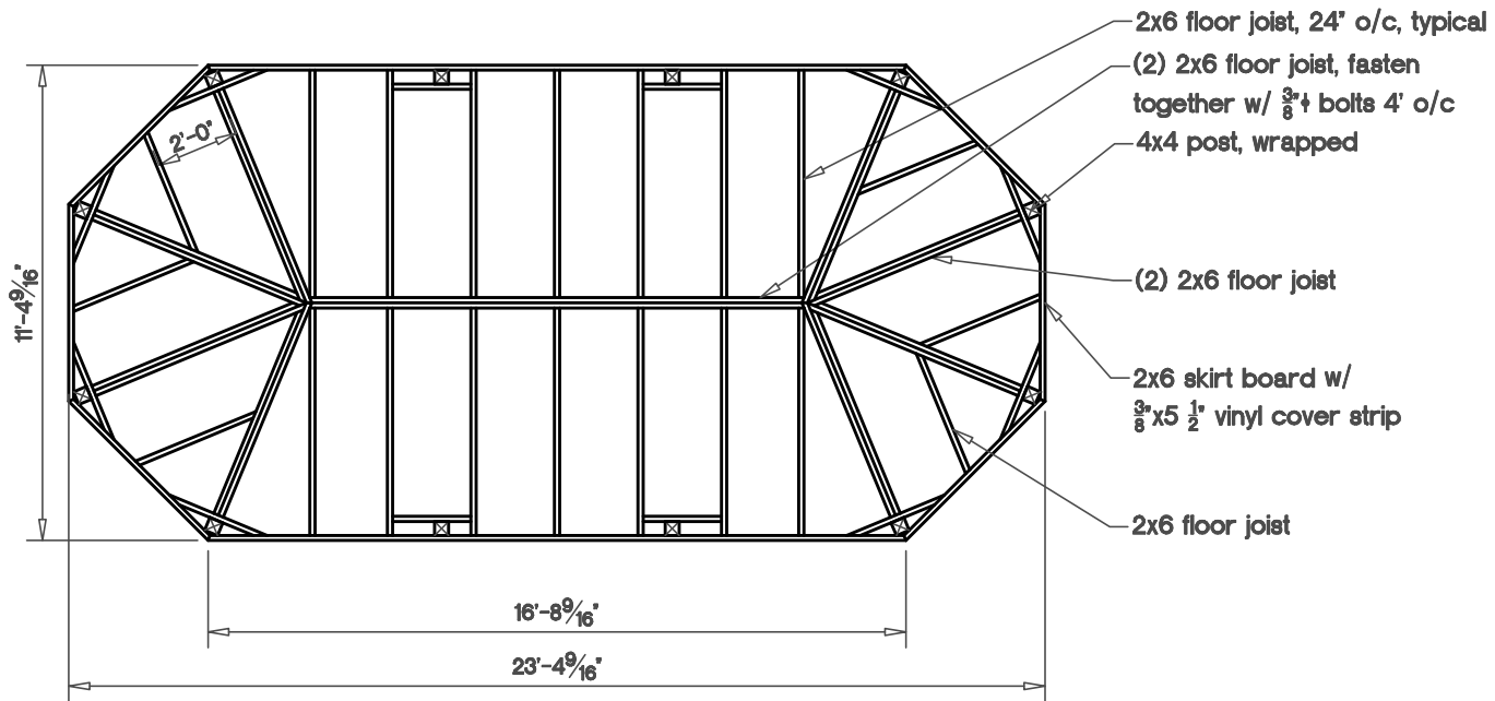
Floor Framing Plan Fully Assembled Unit
