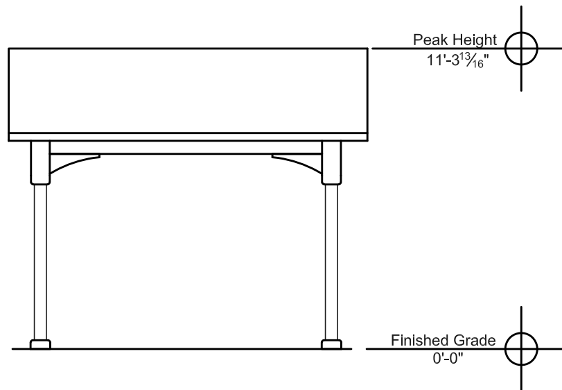
Side Elevation
