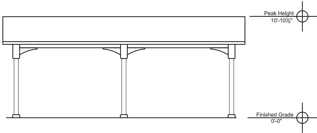
Side Elevation
