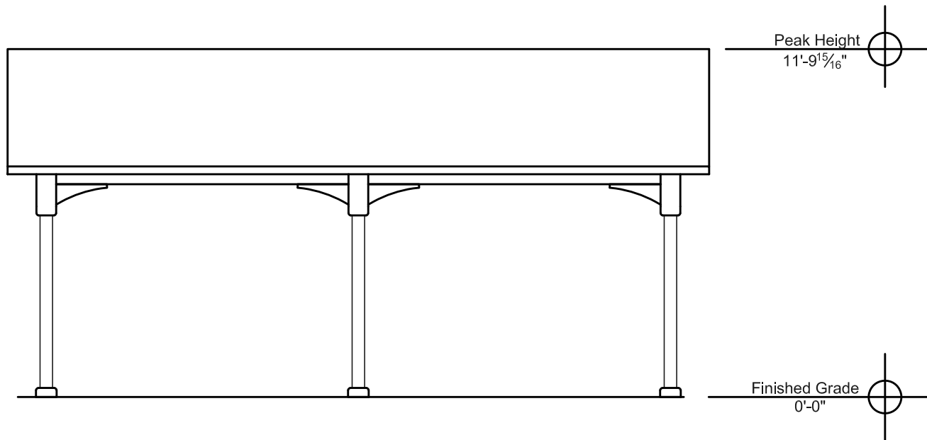
Side Elevation
