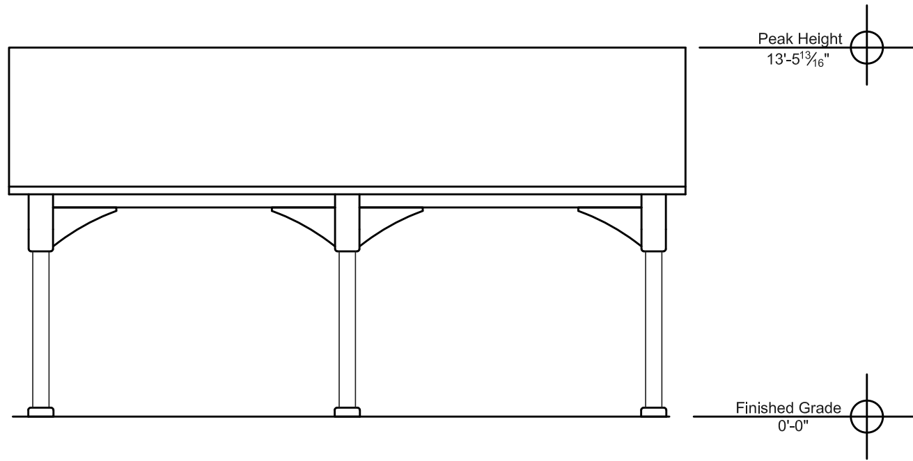
Side Elevation
