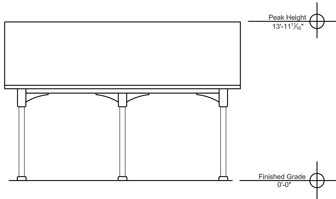
Side Elevation
