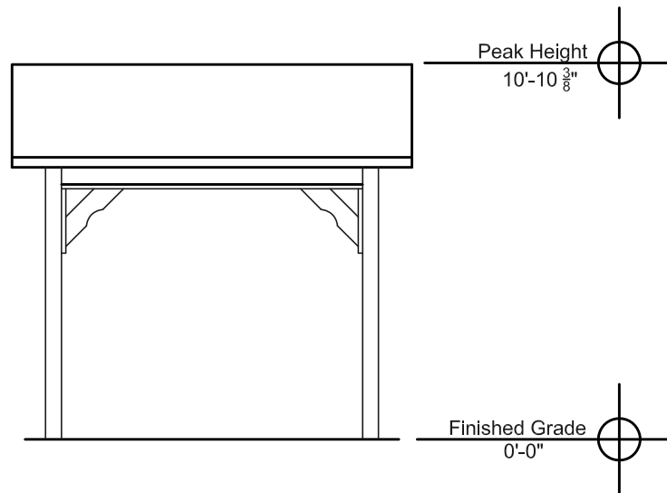
Side Elevation
