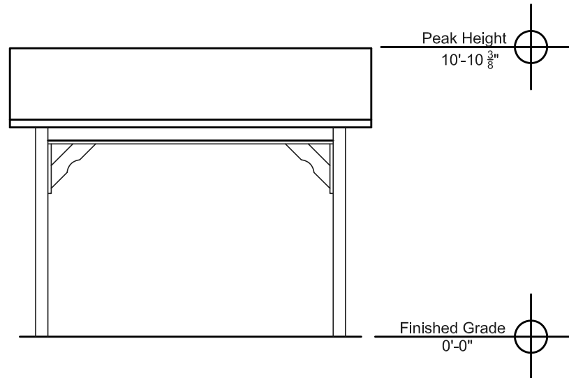
Side Elevation
