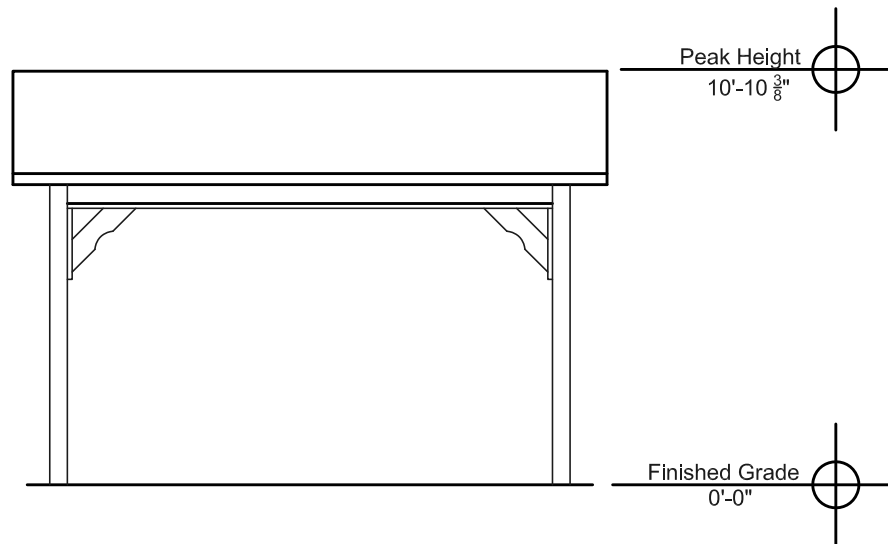
Side Elevation
