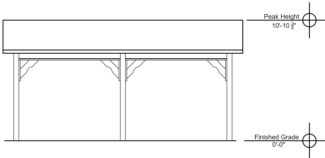
Side Elevation
