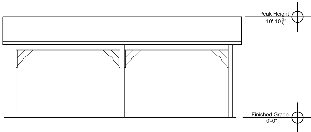
Side Elevation
