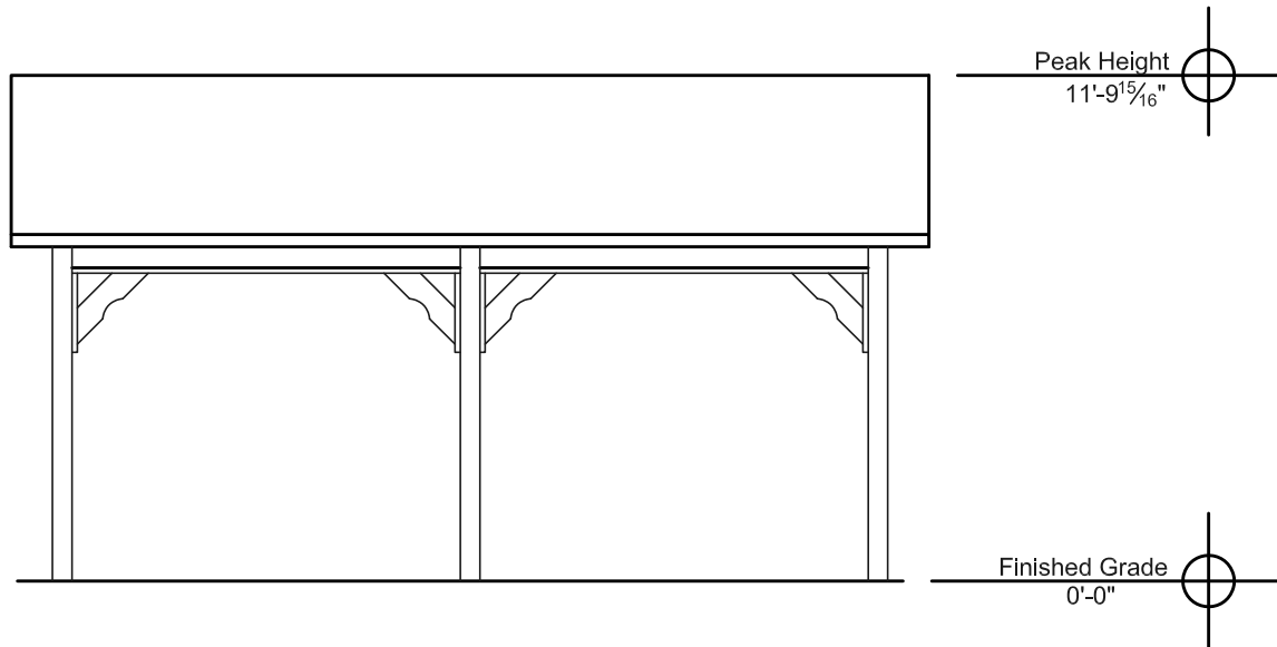
Side Elevation
