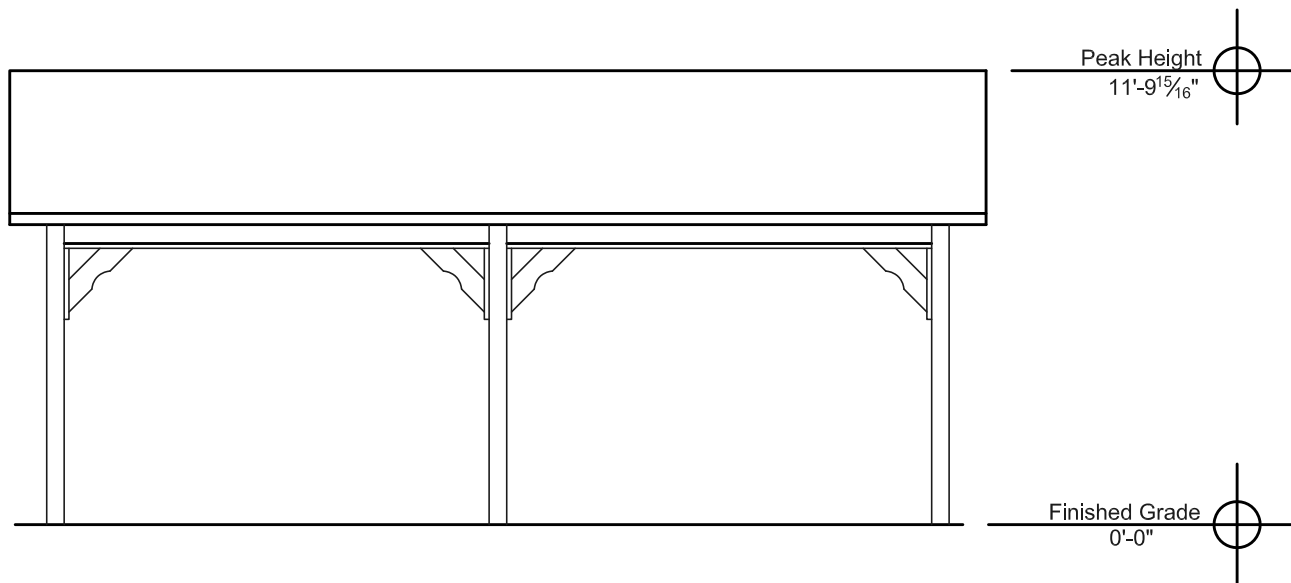
Side Elevation
