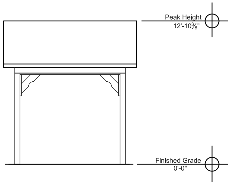
Side Elevation
