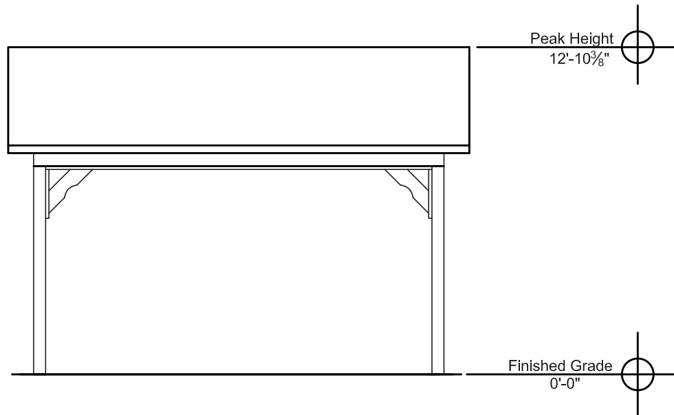
Side Elevation
