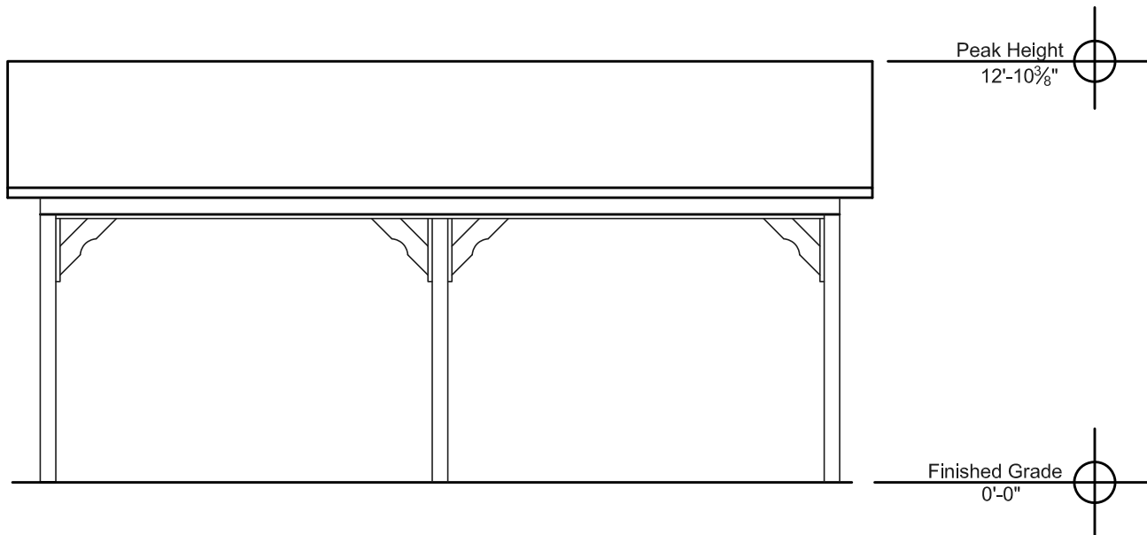
Side Elevation
