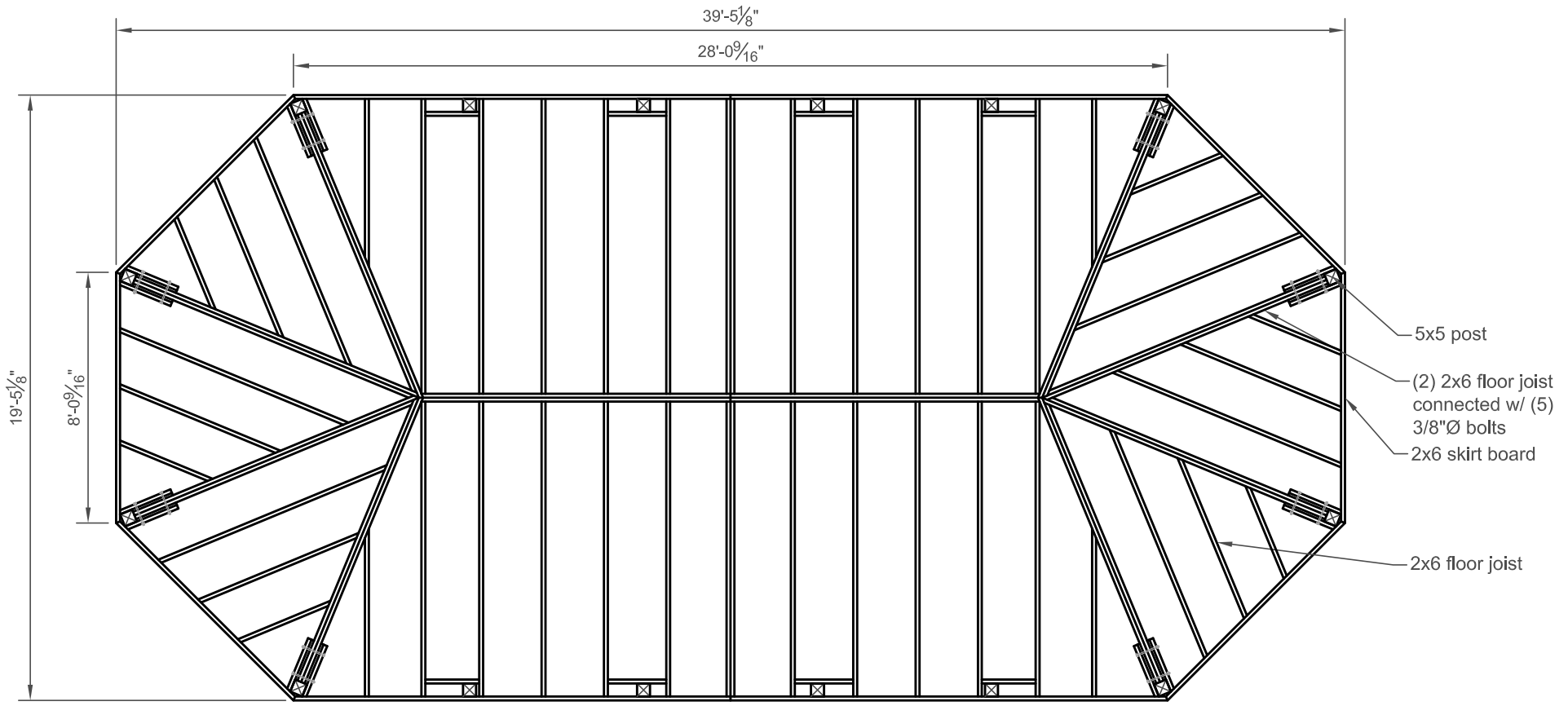
Floor Framing Plan
