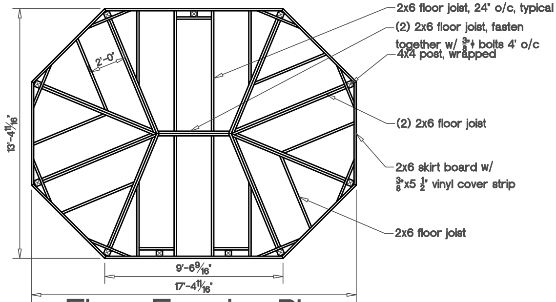
Floor Framing Plan Fully Assembled Unit
