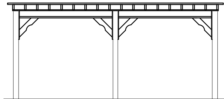
Side Elevation
