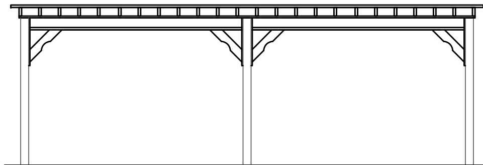
Side Elevation
