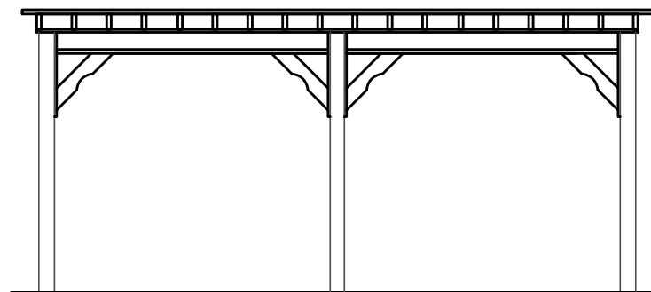
Side Elevation
